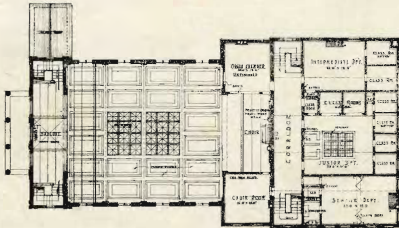
BALCONY FLOOR PLAN SCALE 1/8" = 1'-0"
